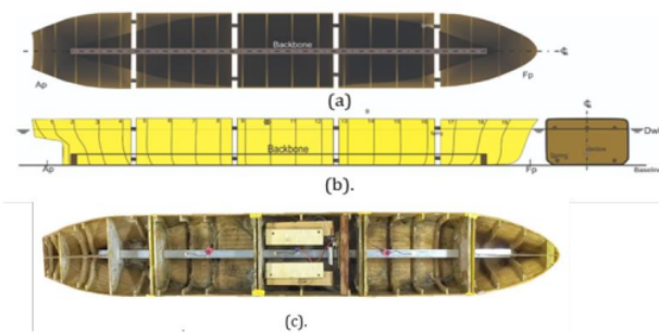
Figure 2 Model of the hydroelastic body: (a) sketch of the segmented model, top view; (b) sketch of the hydroelastic body, side view; and (c) physical model of the hydroelastic body.
