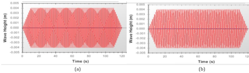
Figure 4 Time history of a wave within 120 sec: (a) wave frequency of 0.92 Hz and a length of 1.83 m; and (b) wave frequency of 0.81 Hz and a length 2.38 m
